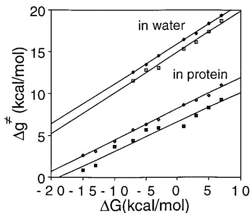
Figure 4. The dependence of the quantum ( \square , \square ) and classical ( \diamond , \blacklozenge ) \Delta g^\ddagger on \Delta G_0 for PT and DT in the active site of carbonic anhydrase and in a solvent cage. In order to focus on the effect of the reorganization of the solvent we included the \text{Zn}^{2+} ion in the solvent cage in addition to the two reacting water molecules (our regular reference reaction does not include the \text{Zn}^{2+} in the reference reaction). This procedure is justified since we are interested in quantum mechanical catalytic effects for the hypothetical case where \Delta G_0 is the same in the enzyme and water reactions. As the figure shows, the activation barriers are much larger in aqueous solution than in the enzyme site, and the quantum corrections are larger in the enzyme than in solution. Also note that the main reason for the difference in \Delta g^\ddagger is the reorganization energies and not the quantum corrections (for \Delta G_0 = 0 the difference between the classical \Delta g^\ddagger is given by the difference in the corresponding values of \lambda/4 ).
